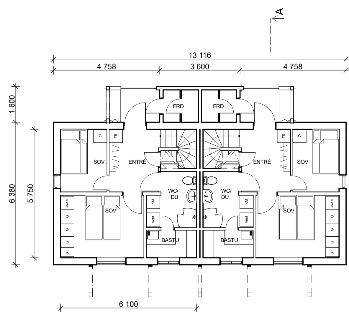
PLAN 1
