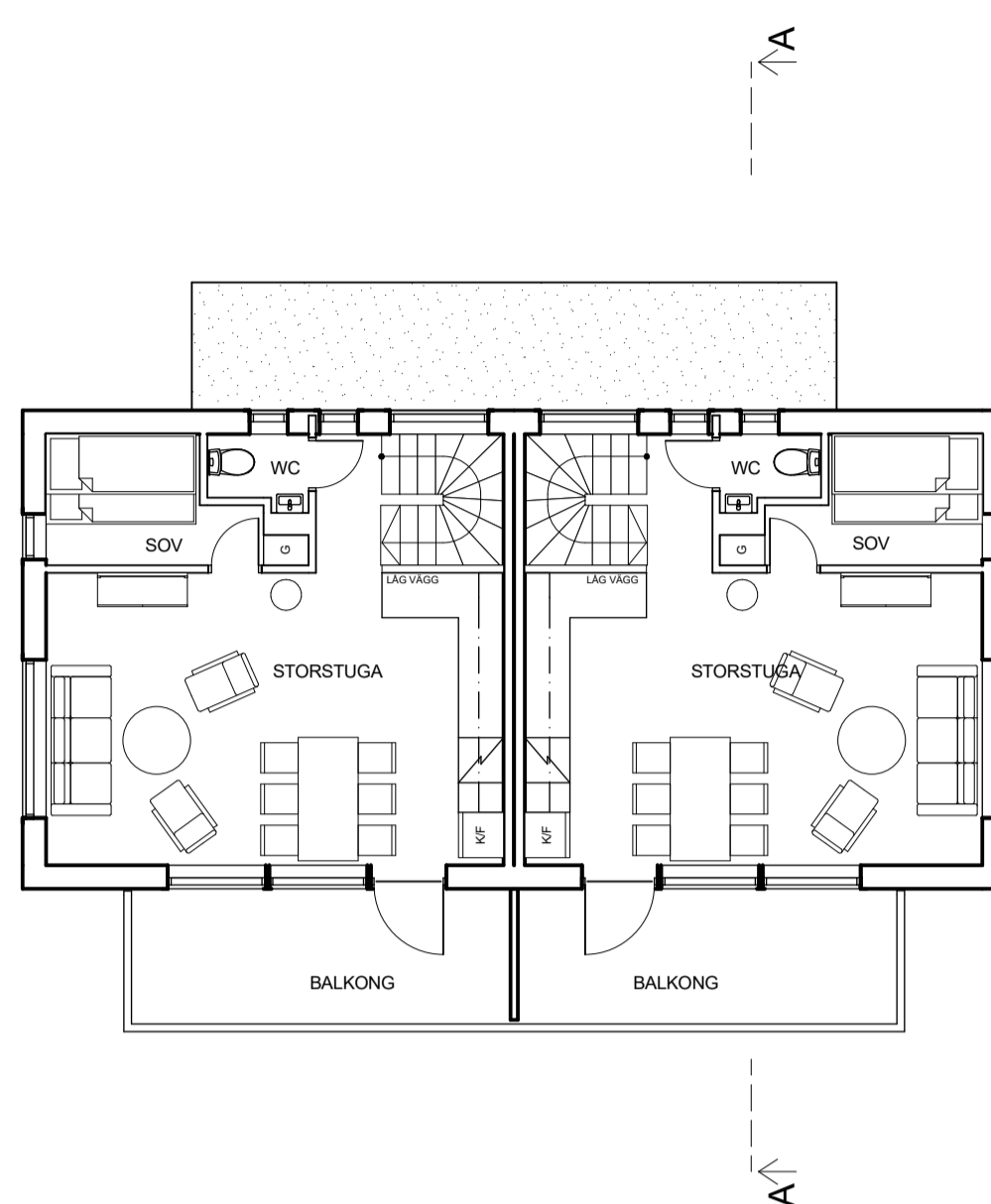
PLAN 2
